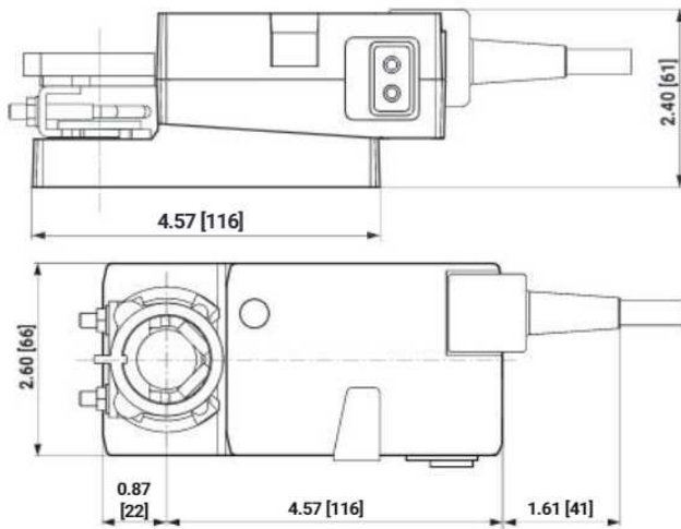
Dimensional drawings LMV-D3-MFT
